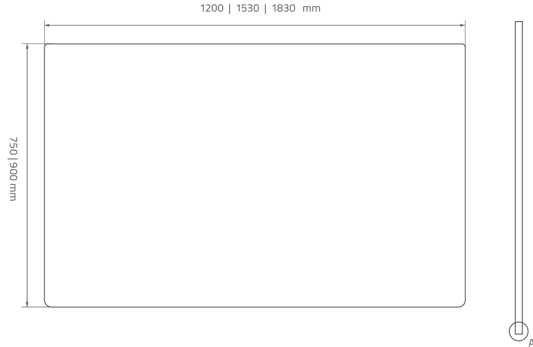
Rectangular HPL worktop with a depth of 750 mm
